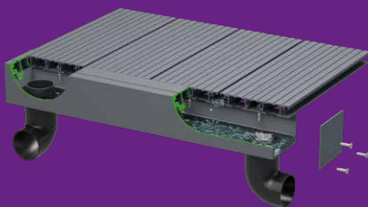
DECK-LEVEL PIPED DRAINAGE
