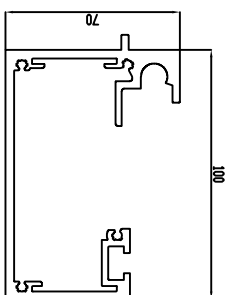
Access Gutter Available 6m long, can be joined SCALE 1:1
