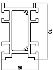
Base Rail Available 6m long, can be joined SCALE 1:1
