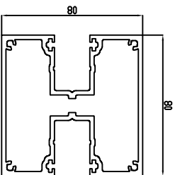
Intermediate Post Available 6m long, can not be joined SCALE 1:1
