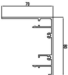
Base Rail Cover Available 6m long, can be joined SCALE 1:1
