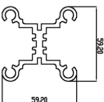
Inter-Post Available 6m long, can not be joined SCALE 1:1
