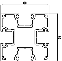
Corner Post Available 6m long, can not be joined SCALE 1:1
