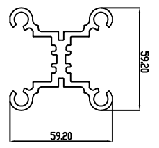
Inter-Post Available 6m long, can not be joined SCALE 1:1
