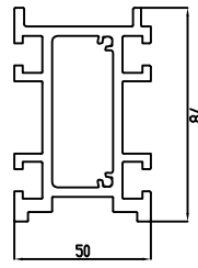
Base Rail Available 6m long, can be joined SCALE 1:1
