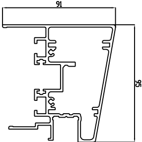
Hand Rail Available 6m long, can be joined SCALE 1:1
