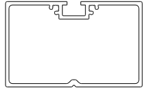
Eco 50 Joist Maximum length: 6000mm SCALE 1:1
