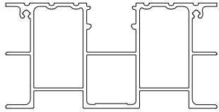
XL Balcony Board Maximum span between fixings: 2000mm Length of extrusion stock: 6m & 4m Can be joined
