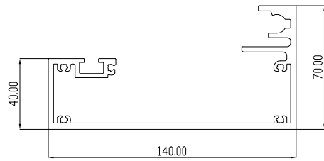
Senior Wide Access Gutter Channel Maximum length: 6000mm Can be joined
