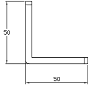
Pedestal Bracket 1 Standard Height: 50mm SCALE: 1:1
