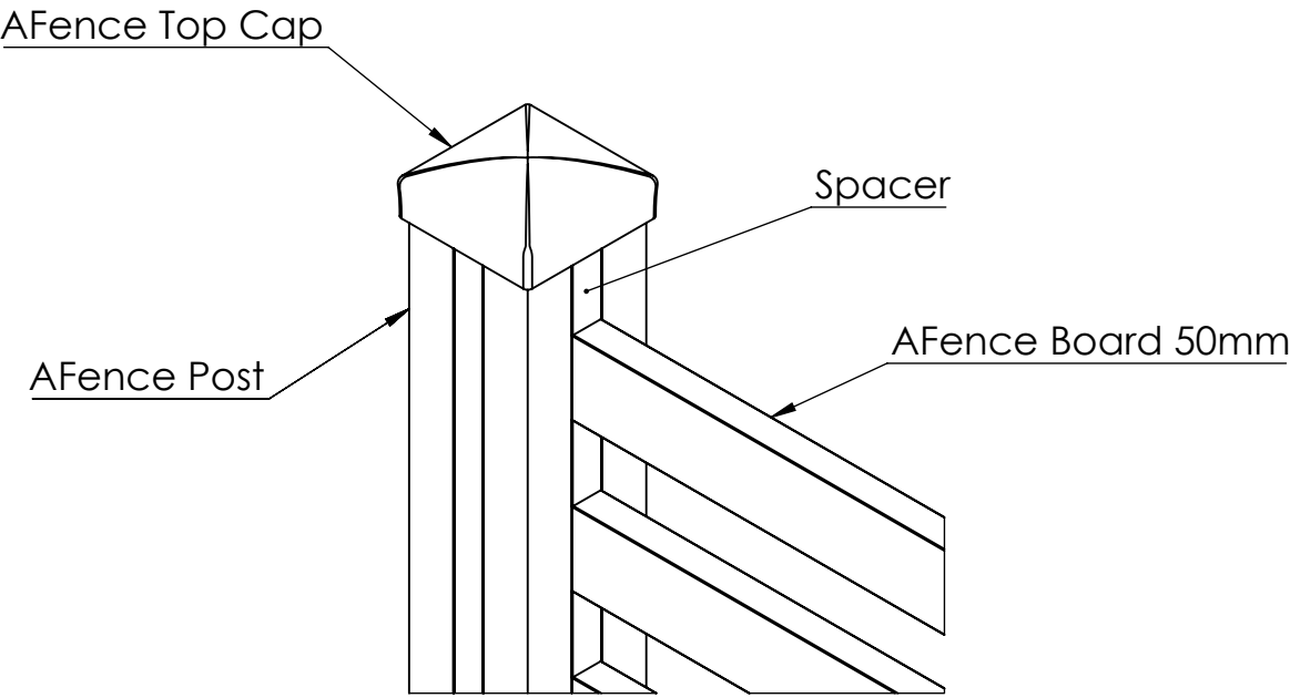
DETAIL A
