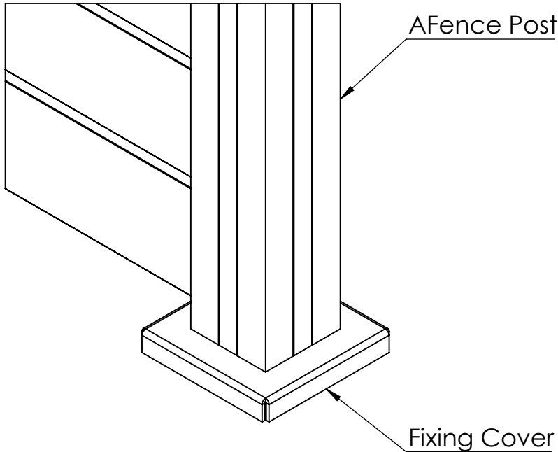
DETAIL B
