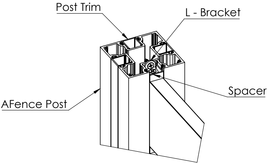
DETAIL F
